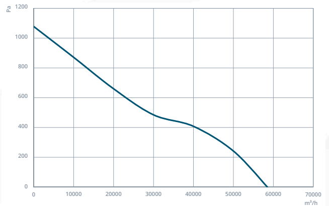
NDTF-SM 1000-8-40
