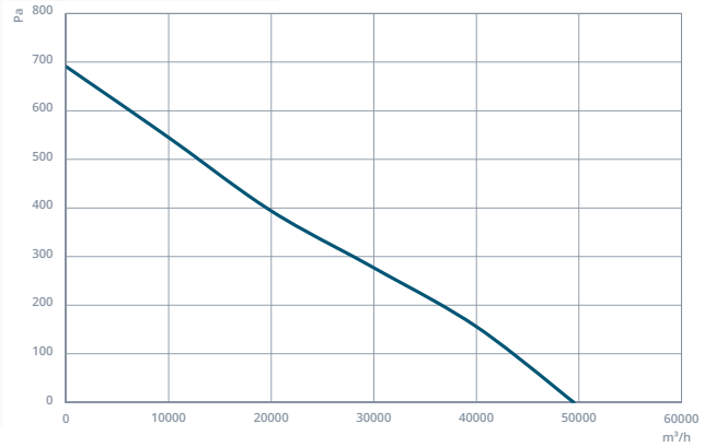
NDTF-SM 1000-5-40
