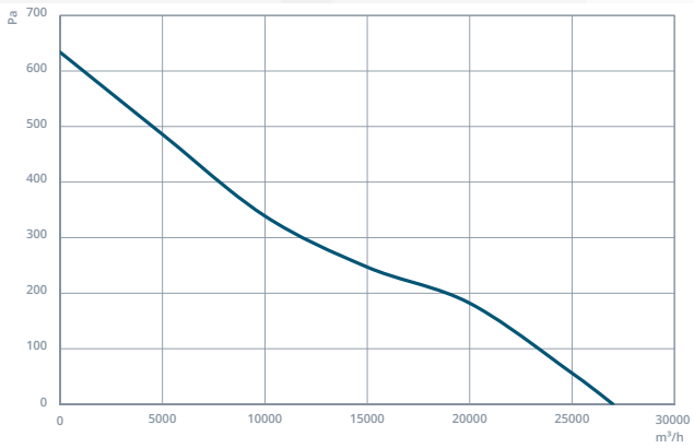
NDTF-SM 800-5-35
