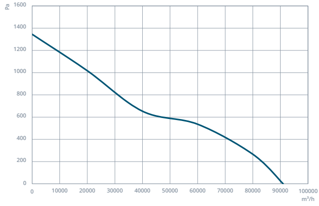
NDTF-SM 1120-8-45
