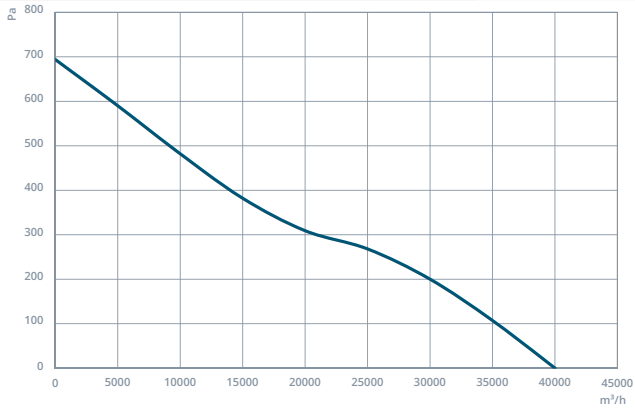
NDTF-SM 900-5-40
