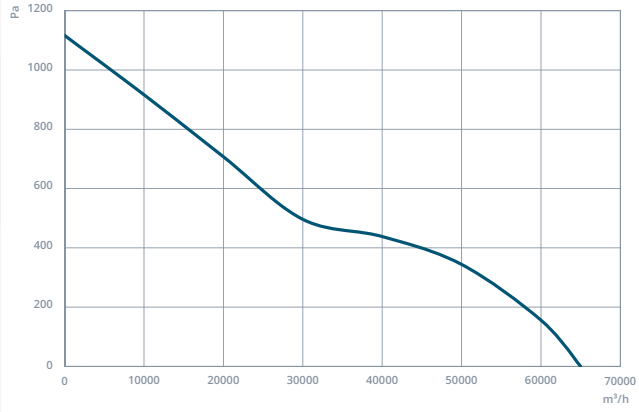
NDTF-SM 1000-8-45
