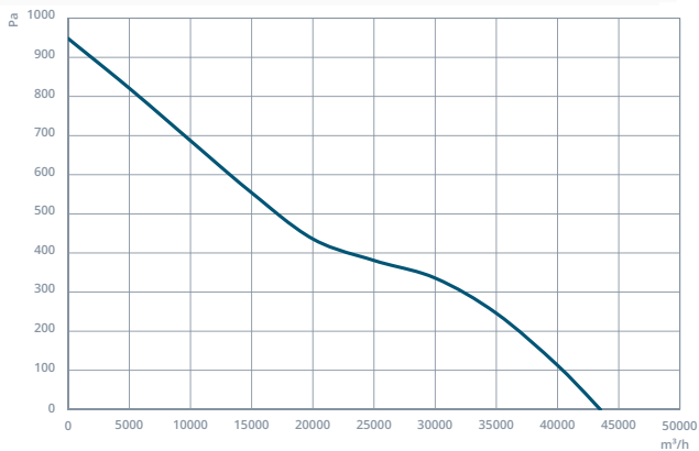
NDTF-SM 900-8-40
