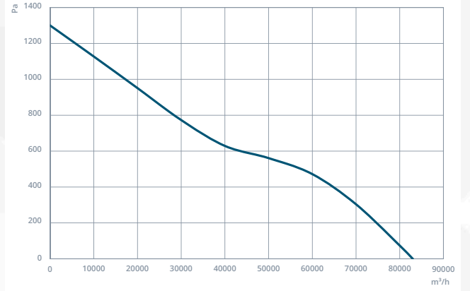
NDTF-SM 1120-8-40
