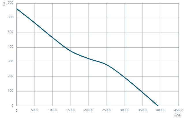
NDTF-DM 900
