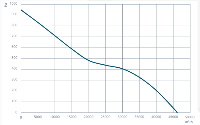
NDTF-DM 900
