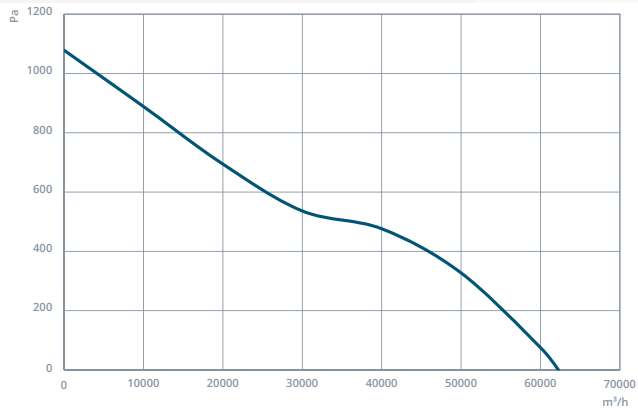
NDTF-DM 1000
