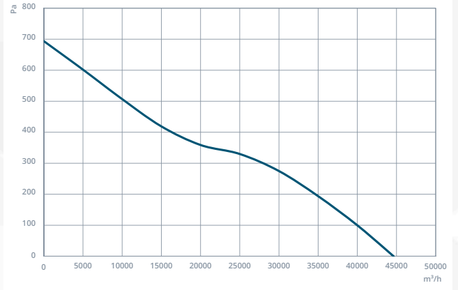
NDTF-DM 900
