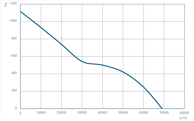
NDTF-DM 1000
