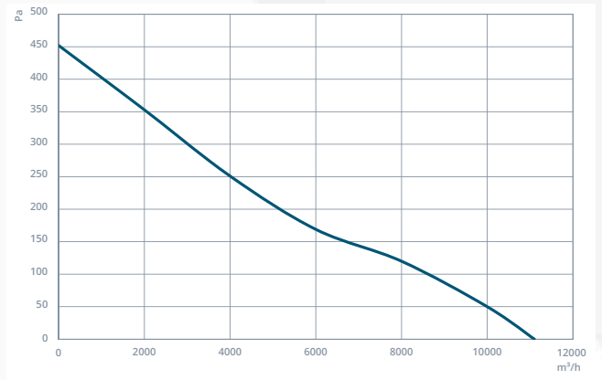
NCF3 630-5-30
