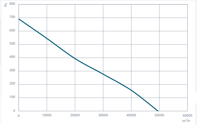
NCF3 1000-5-40
