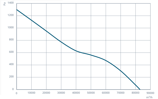
NCF3 1120-8-40
