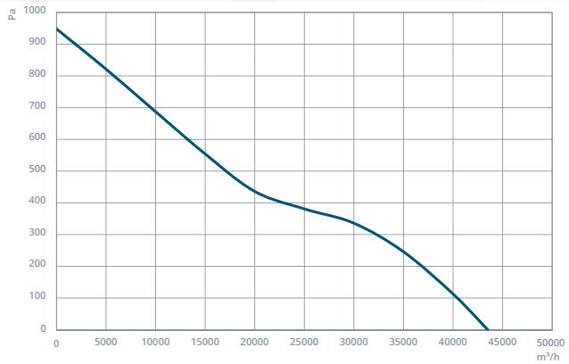
NCF3 900-8-40
