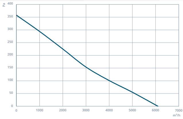
NCF3 560-5-25
