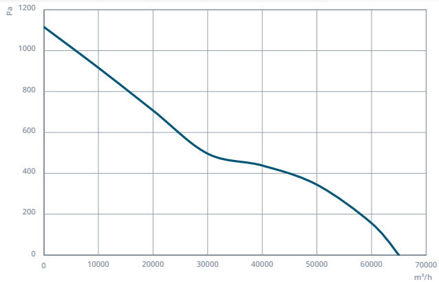
NCF3 1000-8-45
