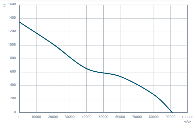
NCF3 1120-8-45
