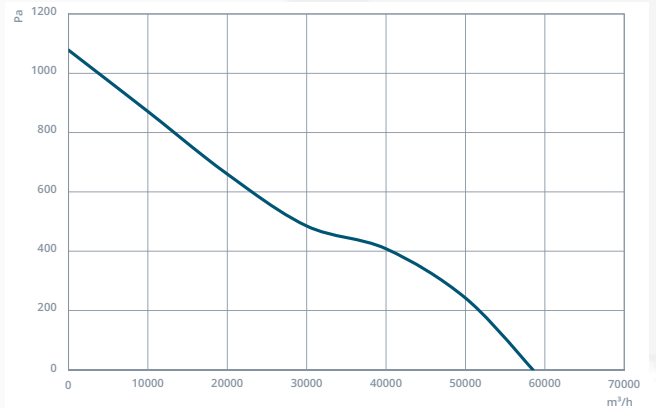
NCF3 1000-8-40
